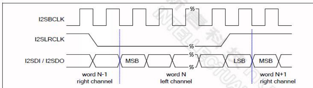
Fig1. I2S Bus Timing Diagram (PCM=0, Format=0)
