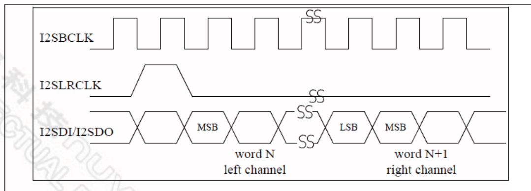
Fig3. PCM A Audio Diagram (PCM=1, Format=0)
